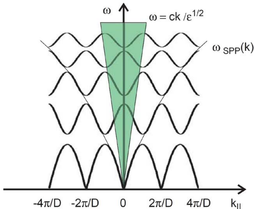
Figure 3- Surface plasmon polarinton dispersion on a periodic structure (periodicity = D) and formation of bandgaps. The dispersion relation on a flat surface is shown by the thin solid line. [15]
